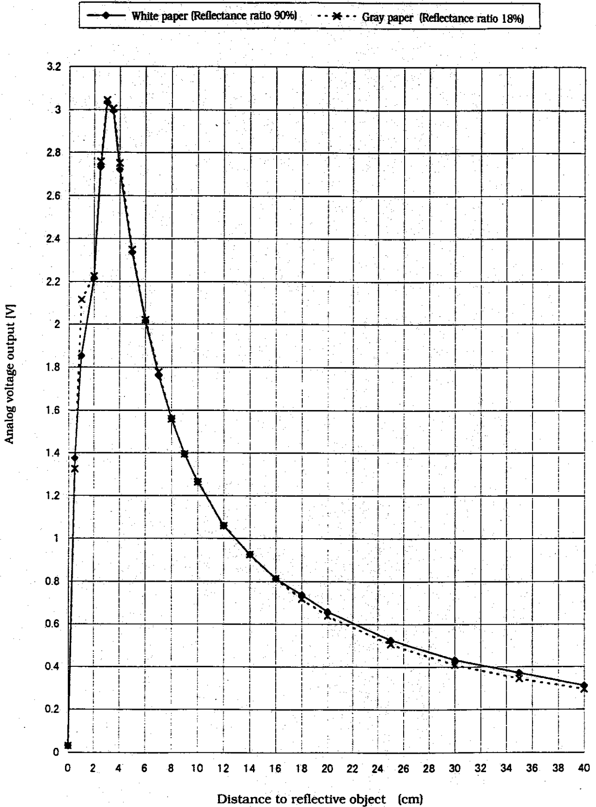
6-1 GP2D120 Example of Output distance characteristics
